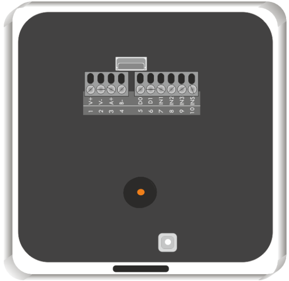
Fig. 8 - connectors on Secustos SQ80 reader models
